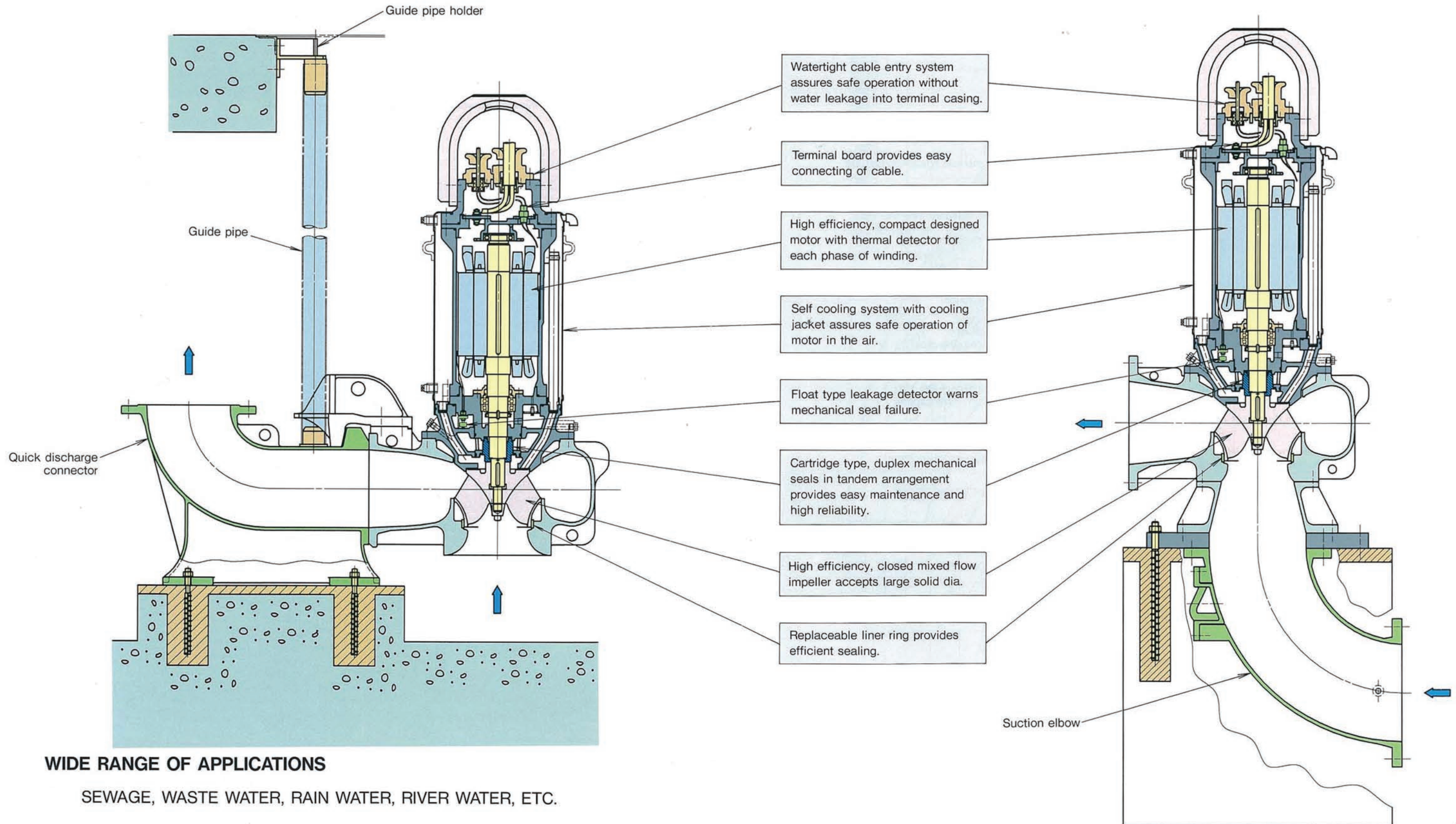
DSCA3 : DRY PIT INSTALLATION
